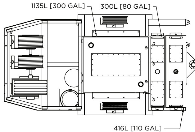
ALTERNATE CONFIGURATION #2 (3) TANK LAYOUT
