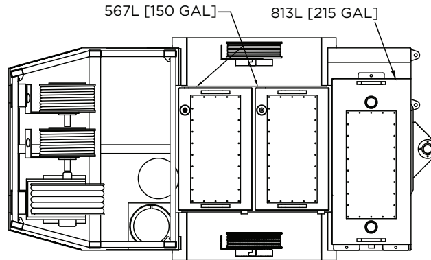
ALTERNATE CONFIGURATION #1 (3) TANK LAYOUT
