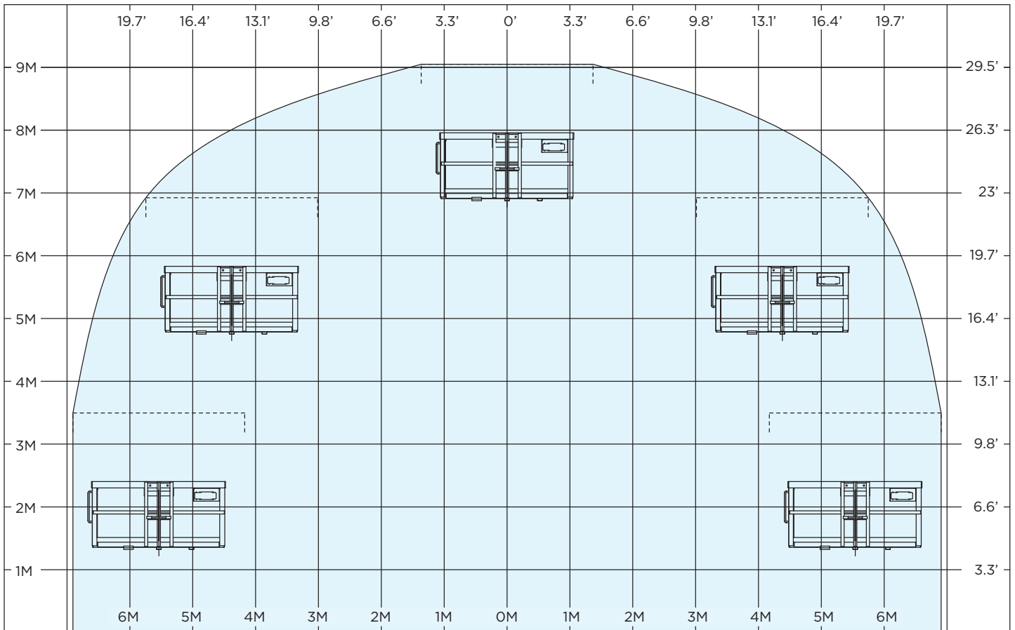
Boom Coverage with Machine 305 mm (12 in) from Face
