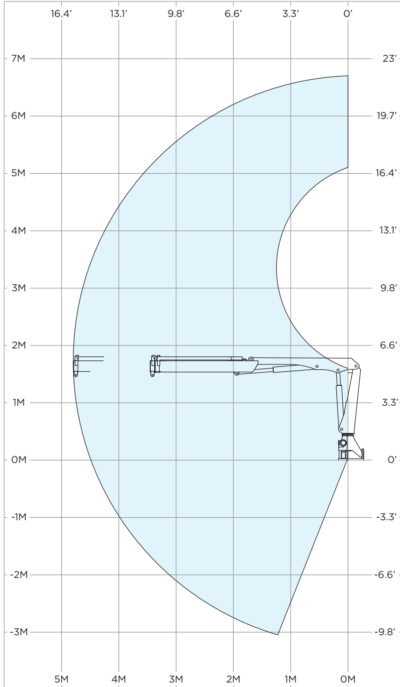
HIAB 044-1 Crane Coverage
